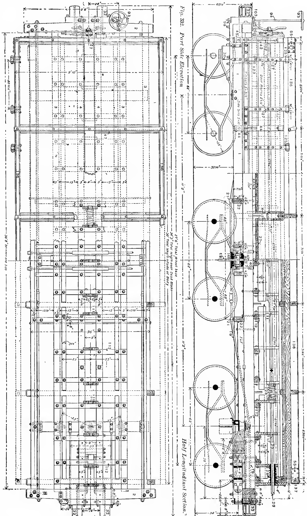
Fig. 333. Half Plan of Floor and Half Plan of Underframe.
